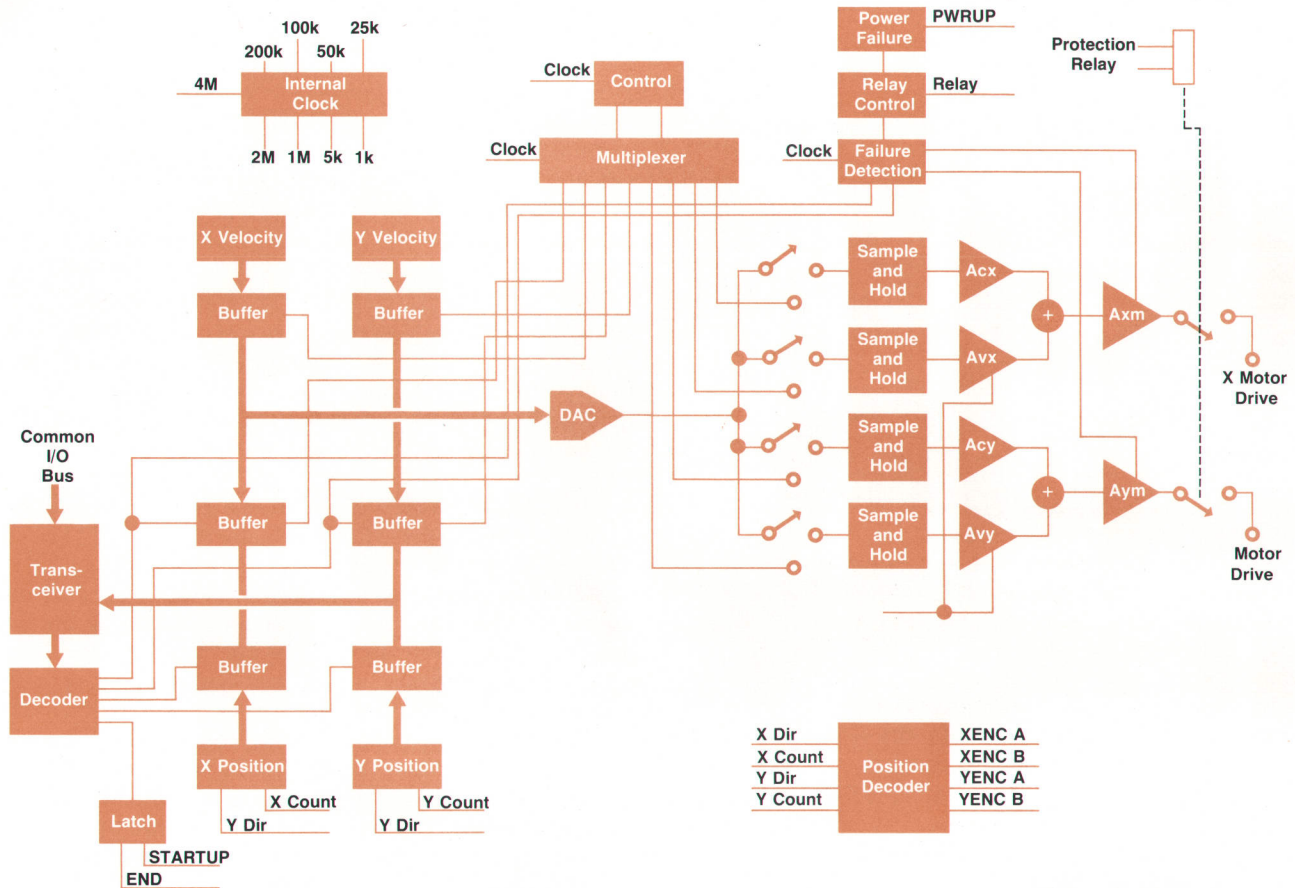
Fig. 3. Block diagram of the 7580A servo control system.
